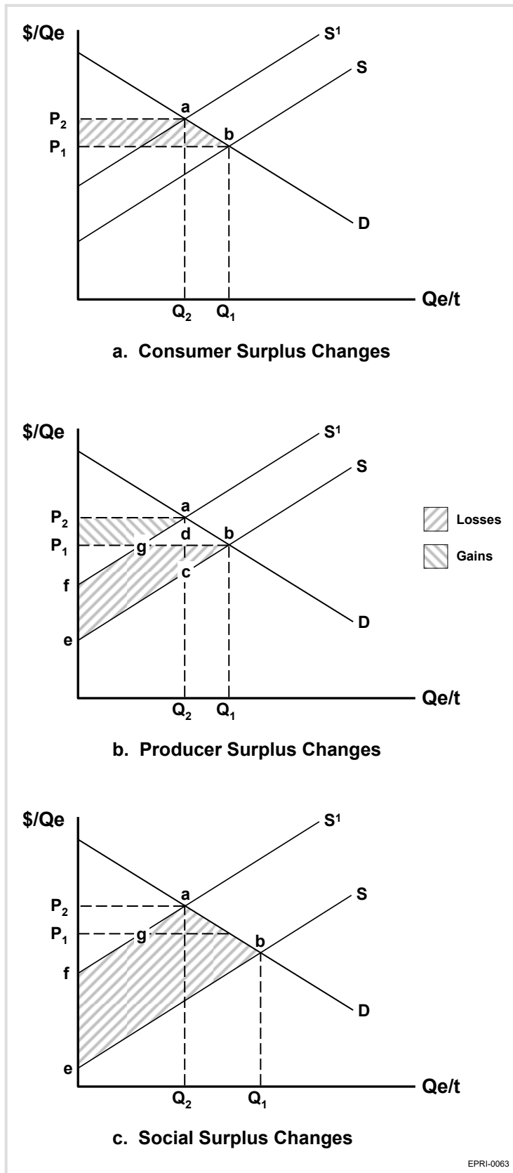
Figure 7.2: Economic Welfare Impacts of a Regulation Requiring Closed-Cycle Cooling
